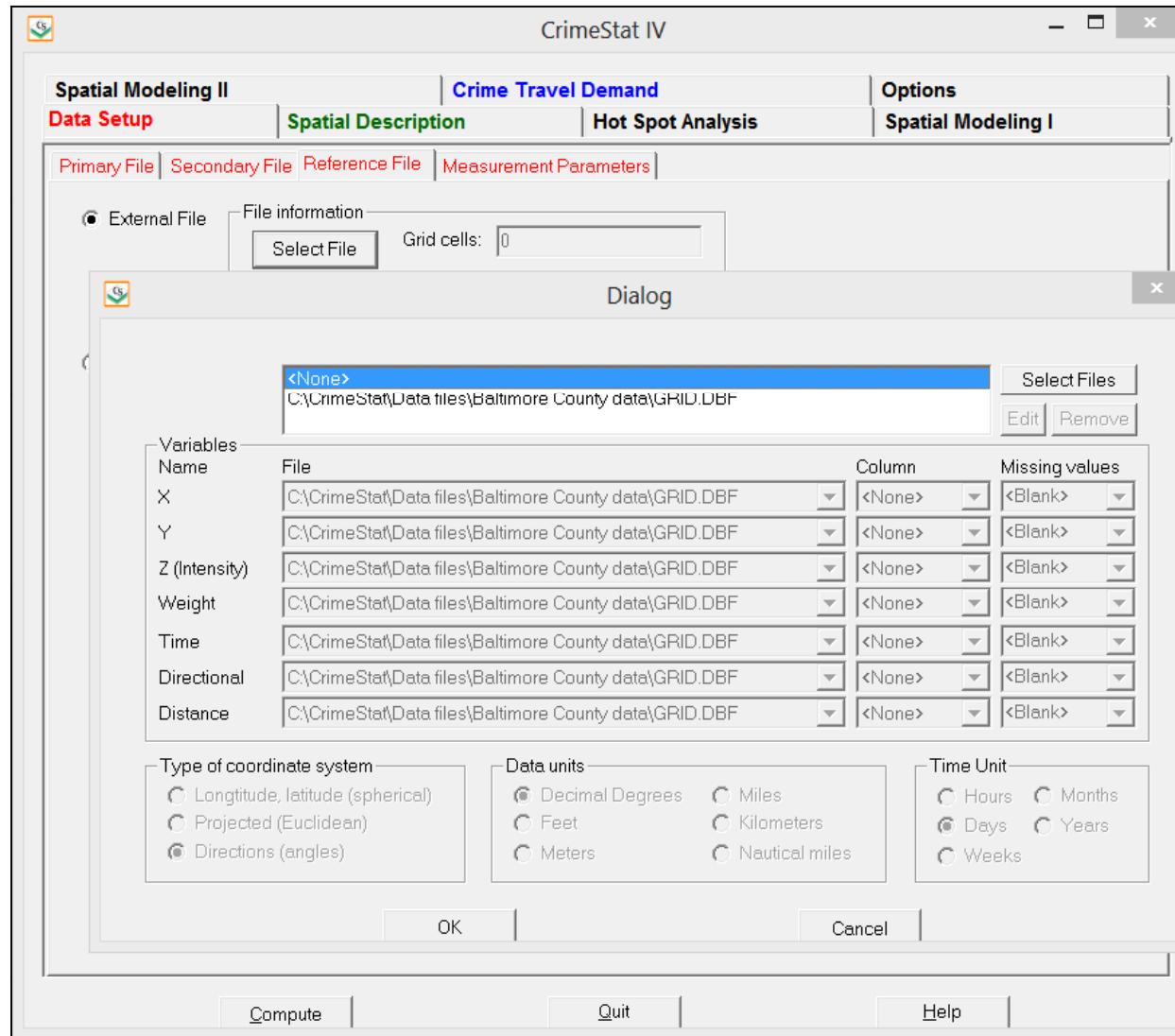
Figure 3.11: Reference File Definition With An External File
