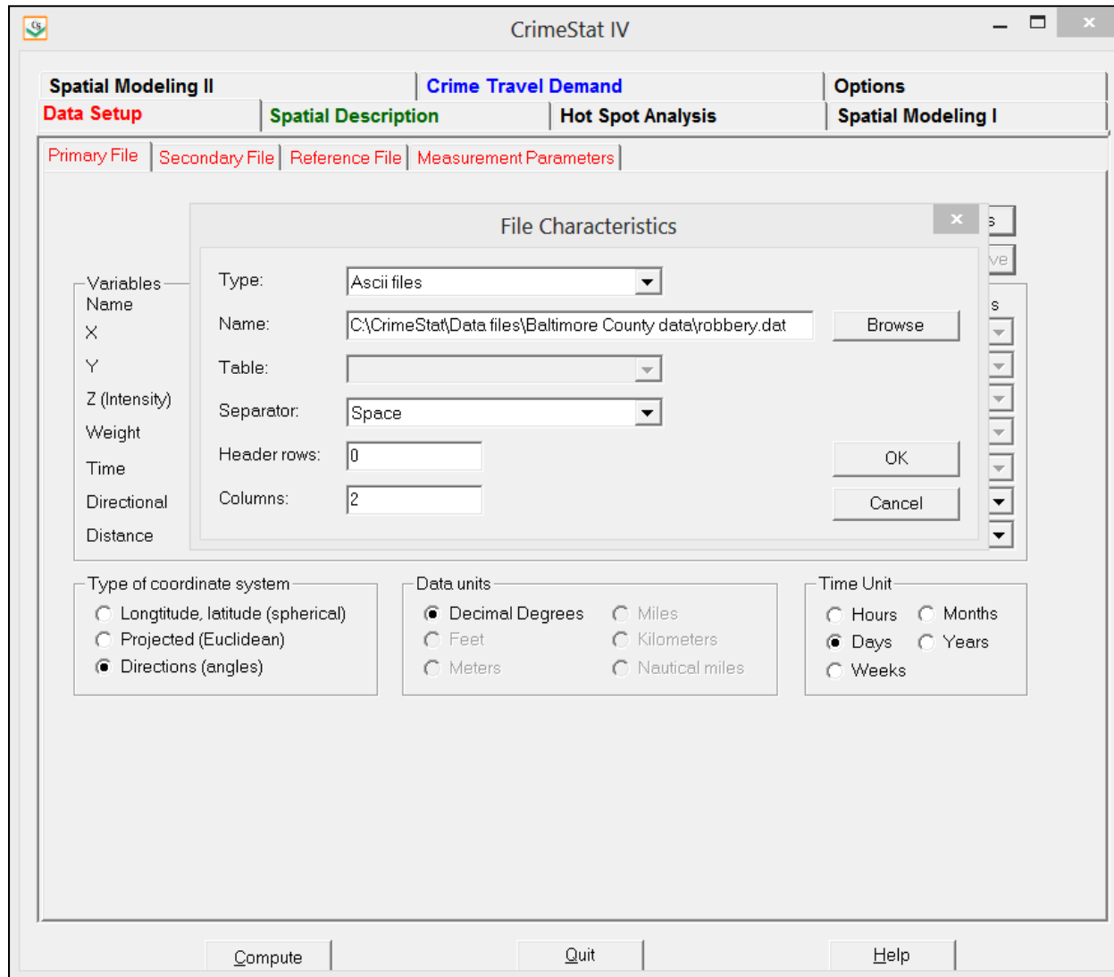
Figure 3.7: Ascii File Selection of Secondary File
